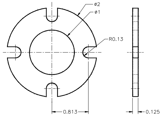
Figure 3 Dimensions of the Disk
