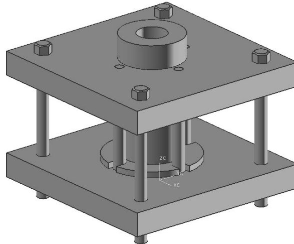
Figure 1 The Fixture assembly
